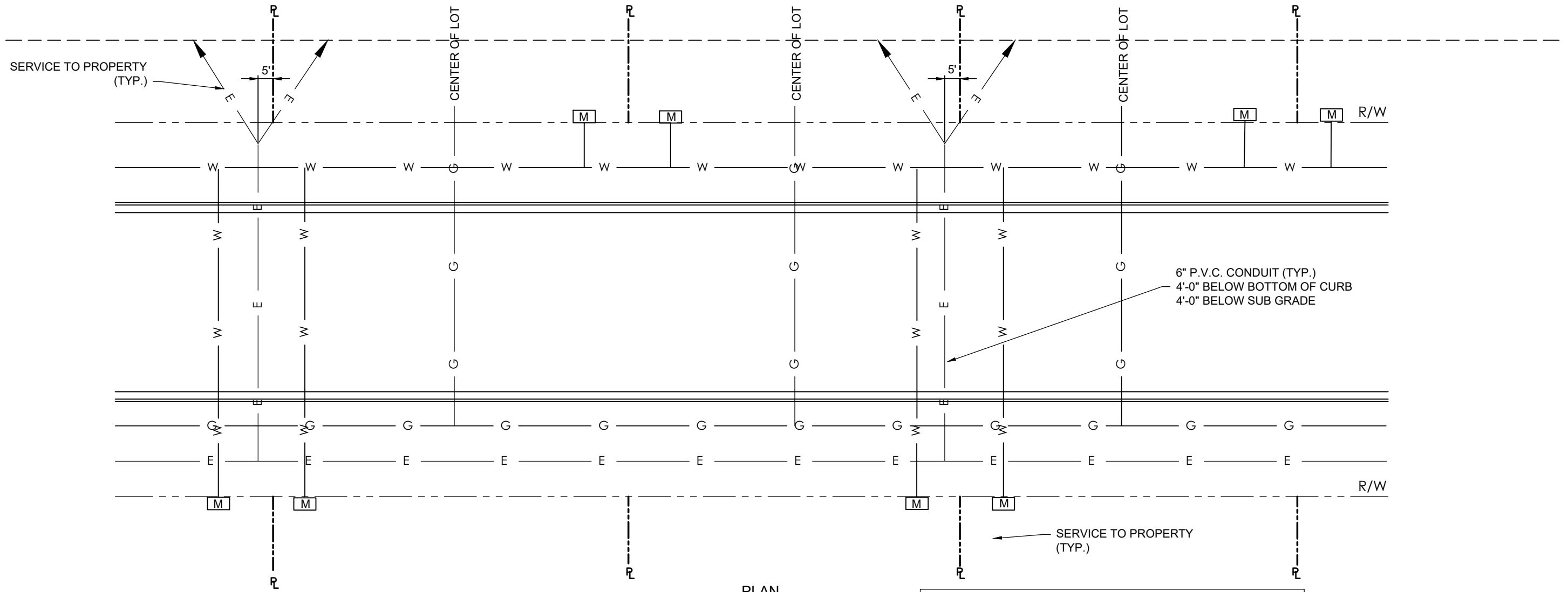
PLAN NTS
