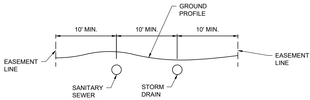
PROFILE NTS
